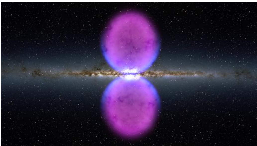
Figure 1: Fermi bubble.[1]
