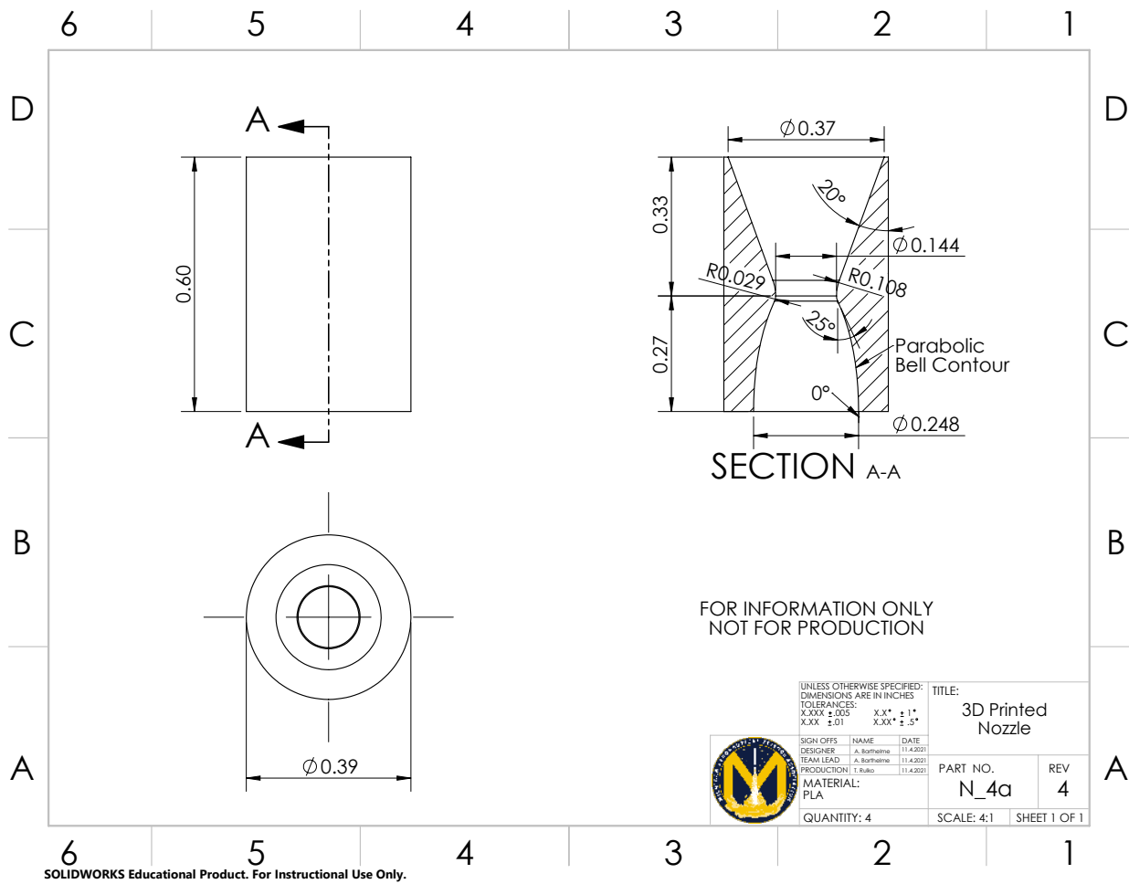
Figure 2: Reference drawing for dimensions of the 3D-printed nozzle.
