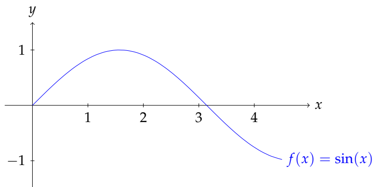
Figure 1.1: Graph of y = \sin(x) .
